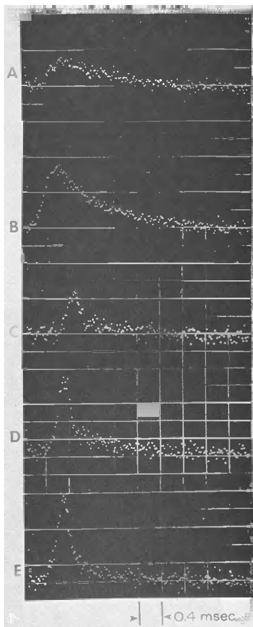
Fig. 4. Time-of-flight distribution for discharged H_2 at m/e = 1 : (A) discharge off, straight-through beam; (B) discharge on, straight-through beam; (C-E) discharge on, direct beam blocked, focussing magnet current 15A (C), 30A (D) and 45A (E), 50 W microwave discharge, P = 0.5 torr.
