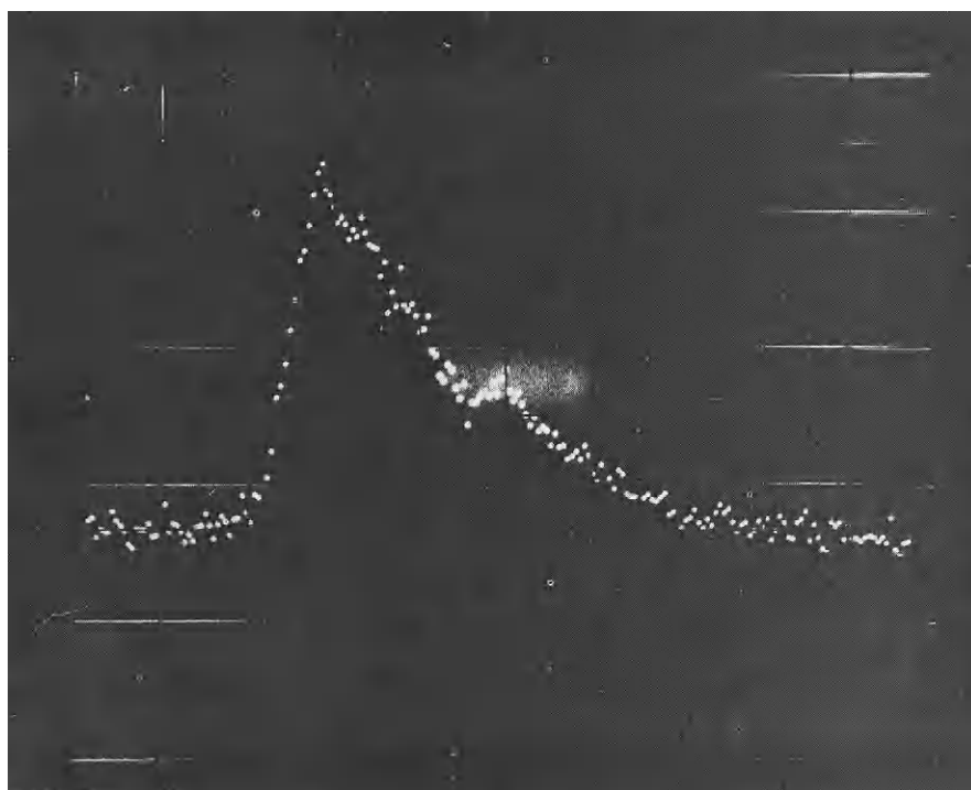
Fig. 5. Time-of-flight distribution of discharged F_2 (8%) in He at m/e = 19 , P = 0.3 torr, 50 W microwave discharge, direct beam blocked, focusing magnet current 40A.
