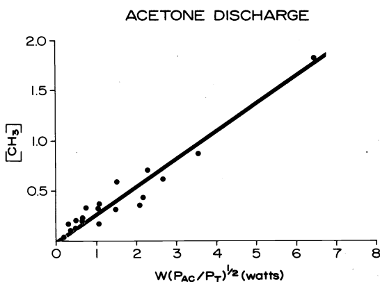
Fig. 7. Relative methyl radical concentrations in an acetone discharge. Variation of variables: W , 1–20 W; P_{acetone} , 0.006–0.038 torr; P_{total}(Ar) , 0.4–0.8 torr.
