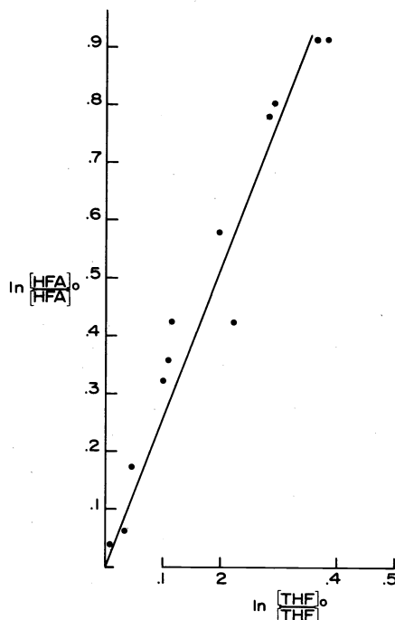
Fig. 9. Two substrate discharge, hexafluoroacetone and tetrahydrofuran, P_{\text{hexafluoroacetone}} \approx 0.0018 torr, P_{\text{tetrahydrofuran}} \approx 0.020 torr, P_T = 0.4-0.8 torr, W = 1.7-12.6 W, \tau \approx 0.025 sec.
