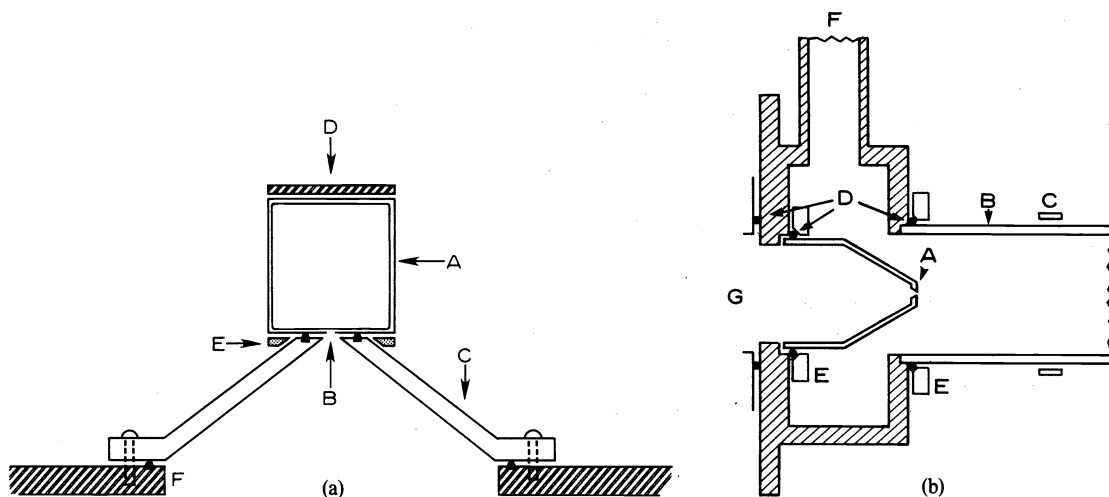
Fig. 6. Arrangements for sampling directly from r.f. discharges. (a) A—square cross-section quartz flow tube; B—sampling orifice; C—mounting cone; D—grounded capacitor plate; E—capacitor plate; F—molecular beam analyzer. (b) A—aluminum oxide sampling cone; B—quartz flow tube; C—r.f. electrode; D—O-ring seals; F—to pump; G—molecular beam analyzer.
