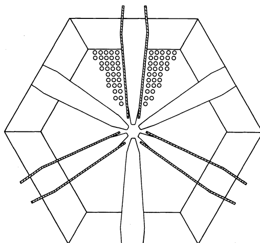
Fig. 2. End view of the hexapolar electromagnetic-electrostatic field. The energizing coils are only shown around one of the pole tips.
