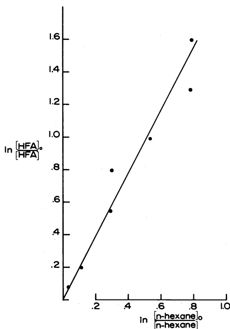
Fig. 10. Two substrate discharge, hexafluoroacetone and n -hexane, P_{\text{hexafluoroacetone}} \approx 0.0035 torr, P_{\text{n-hexane}} \approx 0.017 torr, P_T = 0.5-1.0 torr, W = 1.2-13.2 W, \tau \approx 0.025 sec.
