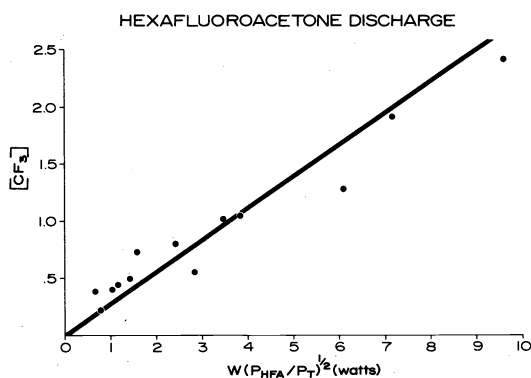
Fig. 8. Relative trifluoromethyl radical concentrations in a hexafluoroacetone discharge. Variation of variables: W , 3–24 W, P_{hexafluoroacetone} , 0.016–0.064 torr; P_{total}(Ar) , 0.4–0.09 torr.
