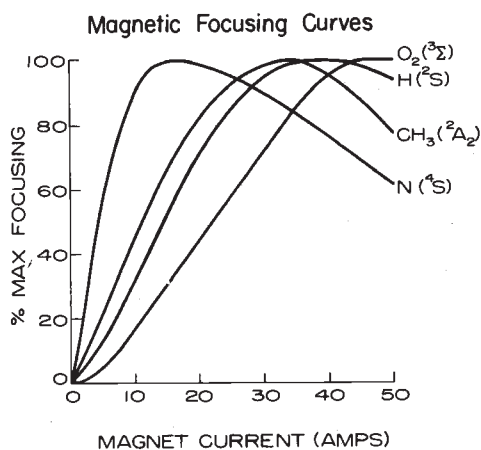
Fig. 3. Relative magnetic focusing of various paramagnetic particles as a function of the energizing current of the hexapolar electromagnet.
