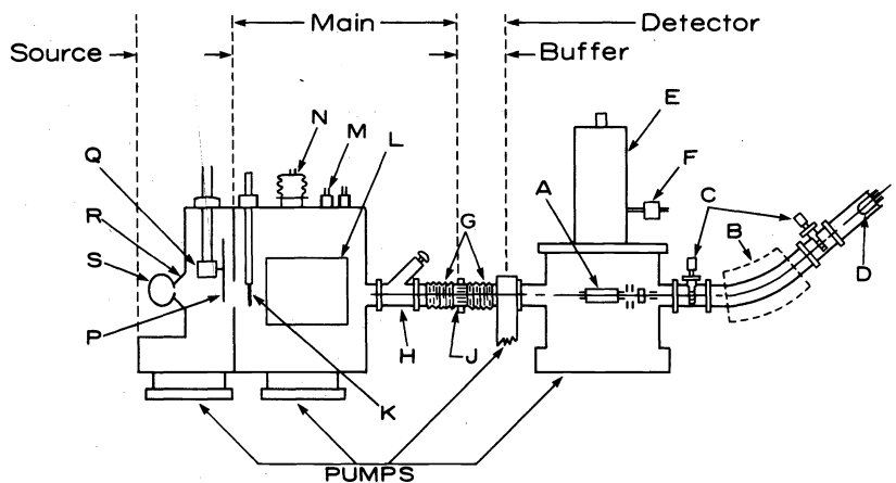
Fig. 1. Side view of molecular beam analyzer; (A) electron bombardment ionizer; (B) magnet pole tips; (C) variable-width slits; (D) electron multiplier; (E) cryopump; (F) variable leak valve; (G) flexible metal bellows; (H) straight-through valve; (J) directional entrance; (K) moveable obstacle; (L) hexapolar electromagnetic-electrostatic field; (M) feed-throughs (9) for water-cooled magnet coils; (N) high-voltage feedthrough; (P) beam modulator or pulsor; (Q) motor; (R) source mounting cone; (S) flowtube; See Ref. 13 for additional details of this apparatus.
