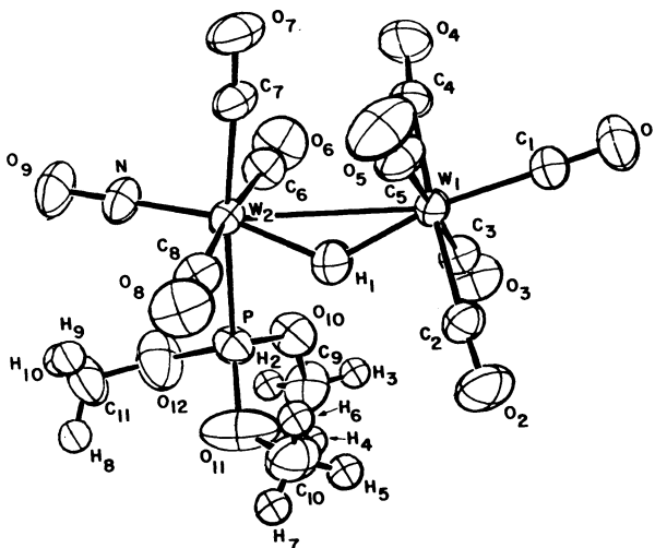
Fig. 7. The structure of \text{HW}_2(\text{CO})_8(\text{NO})(\text{P}(\text{OMe})_3) .
