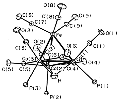
Fig. 11. The structure of \text{HFeCo}_3(\text{CO})_9(\text{P}(\text{OMe})_3)_3 , with methoxy groups removed for clarity,
