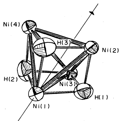
Fig. 12. The central \text{H}_3\text{Ni}_4 core of the \text{H}_3\text{Ni}_4\text{Cp}_4 molecule.
