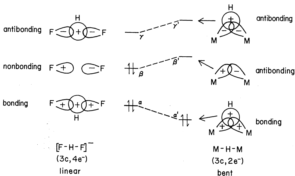
Fig. 10. A schematic comparison between the overlap patterns of linear ( 3c, 4e^- ) and bent ( 3c, 2e^- ) X-H-X systems.
