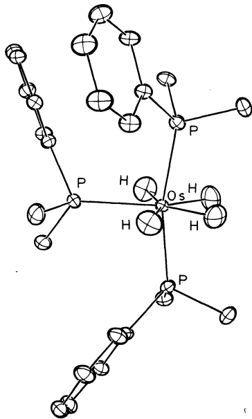
Fig. 1. The pentagonal bipyramidal geometry of H_4Os(PMe_2Ph)_3 . Hydrogen atoms on the methyl and phenyl groups have been omitted for clarity.
