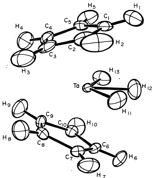
Fig. 5. The structure of H_3TaCp_2 .
