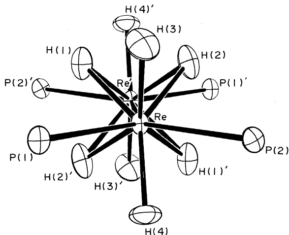
Fig. 4. The skeleton of the H 8 Re 2 (PET 2 Ph) 4 molecule, viewed approximately along the Re-Re axis.
