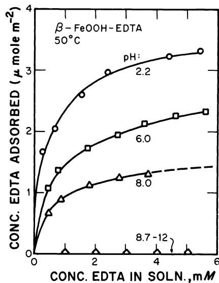
Fig. 8. Adsorption isotherms at 50°C for EDTA on \beta -FeOOH consisting of rod-like particles with an average length of 1 \mu\text{m} and a width of 0.3 \mu\text{m} . Each curve is for a different pH value.
