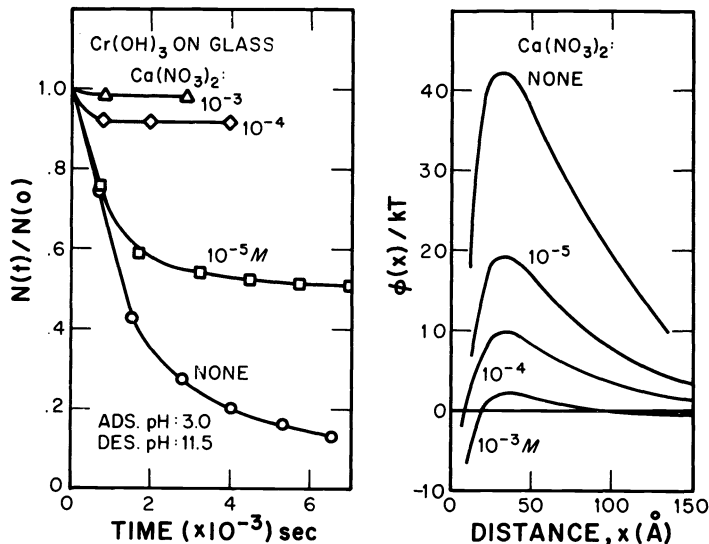
Fig. 15. Left: Fraction of monodispersed spherical chromium hydroxide particles (modal diameter 280 nm) desorbed from glass on repeated elution with rinse solutions of pH 11.5 in the absence (○) and in the presence of 10^{-5} (□), 10^{-4} (◇), and 10^{-3}\text{ M} \text{Ca(NO}_3)_2 . The particles were adsorbed on the glass from a sol at pH 3. Right: Calculated potential energy curves as a function of distance using the sphere-plate model (Eqs. 2 and 4) for the same systems shown left.
