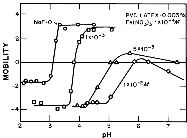
Fig. 13. Electrokinetic mobilities as a function of pH of the same PVC latex as in Figure 12 in the presence of 1 \times 10^{-4} M \text{Fe}(\text{NO}_3)_3 (O) to which 1 \times 10^{-3} (□), 5 \times 10^{-3} (Δ), and 1 \times 10^{-2} M (◇) NaF was added, respectively.
