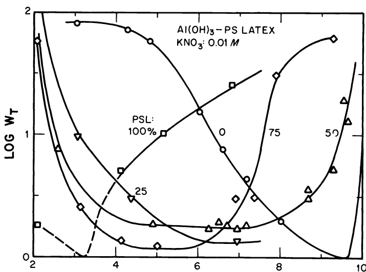
Fig. 10. Total stability ratio, W_T , as a function of pH for a pure aluminum hydroxide sol (modal diameter 570 nm) (○), a pure polystyrene latex (PSL, modal diameter 380 nm) (□), and for mixtures of the two sols containing 25% (▽), 50% (△) and 75% (◇) PSL particles (in terms of number concentration).
