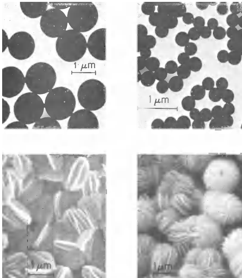
Fig. 2. Transmission and scanning electron micrographs of particles precipitated from various aluminum salt solutions. (a) Amorphous aluminum hydroxide (solution 0.0020 M in Al_2(SO_4)_3 , pH 4.0 aged for 48 hr at 97^\circ C ). (b) Variscite, AlPO_4 (solution 0.050 M in Al(NO_3)_3 and Na_2HPO_4 and 0.035 M in HNO_3 aged for 20 hr at 97^\circ C ). (c) and (d) Boehmite, \alpha-AlOOH (solutions of 0.0050 M in AlCl_3 and 0.0030 M in Al(ClO_4)_3 , respectively, aged for 12 hr at 125^\circ C ).
