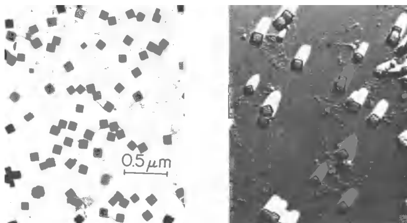
Fig. 3. Electron micrograph and a replica of \text{Co}_3\text{O}_4 spinel particles obtained by heating a 0.010 M Co(II)-acetate solution for 4 hr at 100 C.
