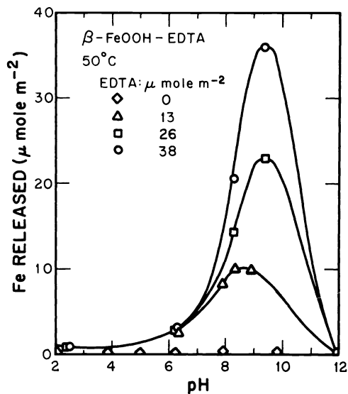
Fig. 9. Solubility of \beta -FeOOH (expressed as released iron) in the absence and in the presence of EDTA in different concentrations as a function of pH at 50°C.
