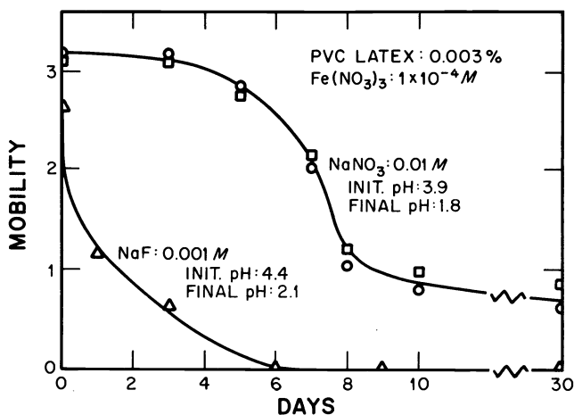
Fig. 14. The change of electrokinetic mobilities ( \mu\text{m}/\text{sec}/\text{V}/\text{cm} ) as a function of time (days) of the same PVC latex as in Figure 12 on acidification of a sol containing 1 \times 10^{-4} M \text{Fe}(\text{NO}_3)_3 . Circles and squares represent systems to which HCl and \text{HNO}_3 , respectively, were added to lower the pH in the presence of 0.01 M \text{NaNO}_3 ; triangles represent systems the pH of which was lowered by \text{HNO}_3 in the presence of 0.0010 M \text{NaF} prior to aging.
