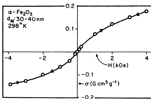
Fig. 5. Magnetization at 298°K as a function of applied field of spherical \alpha -Fe 2 O 3 particles having modal diameters of 30-40 nm.
