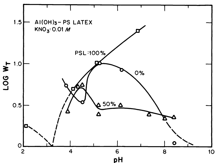
Fig. 11. Analogous plot as Figure 10 except that the aluminum hydroxide particles contained some sulfate ions.
