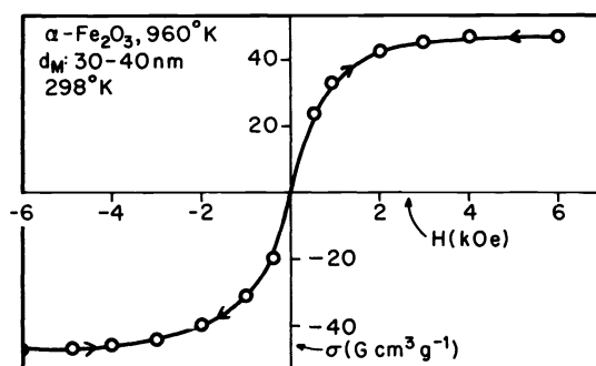
Fig. 6. Magnetization at 298°K as a function of applied magnetic field of spherical \alpha -Fe 2 O 3 particles having modal diameters of 30-40 nm after heat treatment at 960°K in a He atmosphere of 500 torr.
