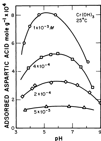
Fig. 7. The total amount of aspartic acid sorbed on spherical chromium hydroxide particles (modal diameter 350 nm) as a function of pH using different initial concentrations of aqueous solutions of the amino acid.
