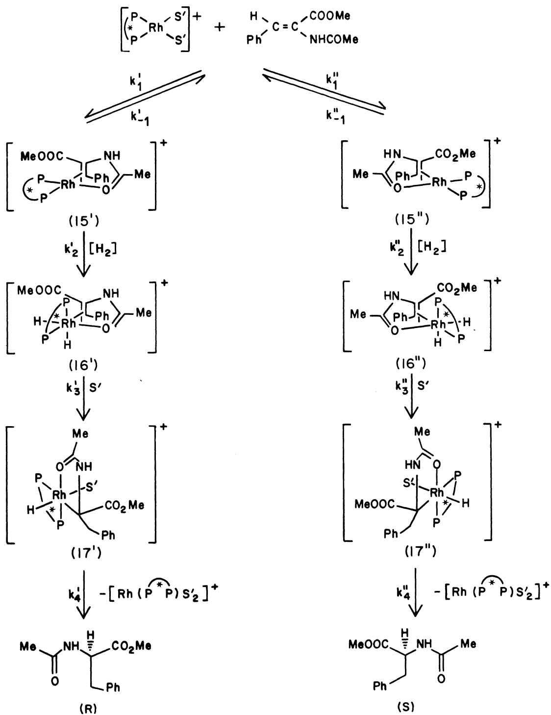
Fig. 2. Mechanistic scheme for the hydrogenation of a prochiral substrate (MAC) with a catalyst containing a chiral chelating diphosphine ligand. ( P^*P = CHIRAPHOS or DIPAMP; S' = methanol.)
