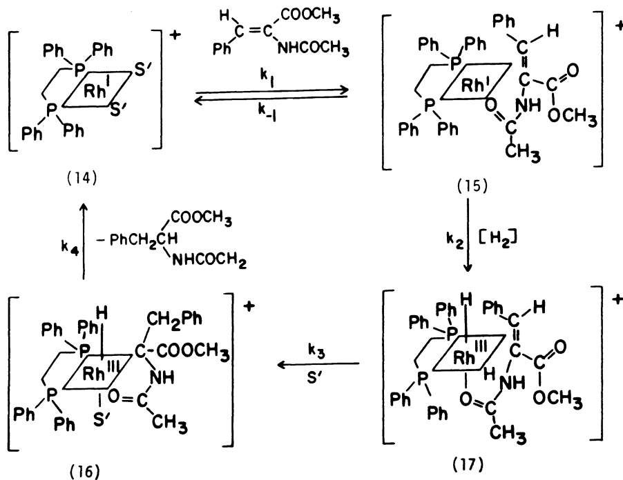
Fig. 1. Mechanism of the [Rh(DIPHOS)] + -catalyzed hydrogenation of methyl-(Z)- \alpha -acetamidocinnamate (MAC).
