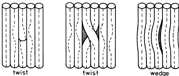
Disclinations in polymers
