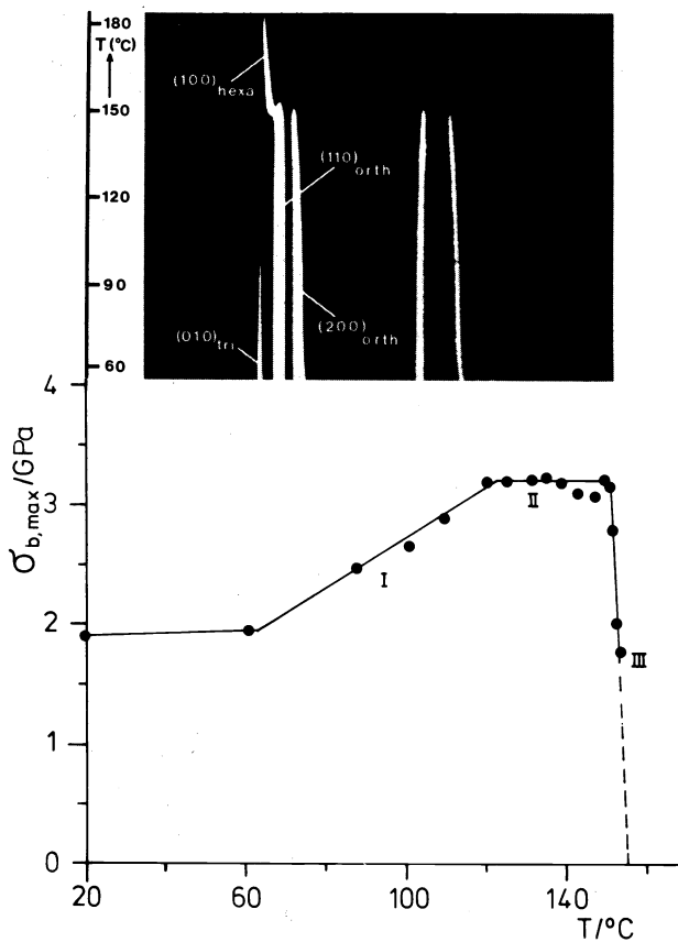
Fig. 8. The lower part shows the tensile strength at break \sigma_b after hot-drawing of "surface-growth" fibers as a function of drawing temperature. The upper part shows an equatorial wide-angle X-ray diffractogram of a constrained "surface-growth" fiber continuously recorded at increasing temperature. The heating rate was 0.35°C/min. Note the transition of the orthorhombic (110) and (200) reflections into the (100) reflection of the hexagonal phase at 150°C, which results in a drastic decrease of the tensile strength upon hot-drawing.
