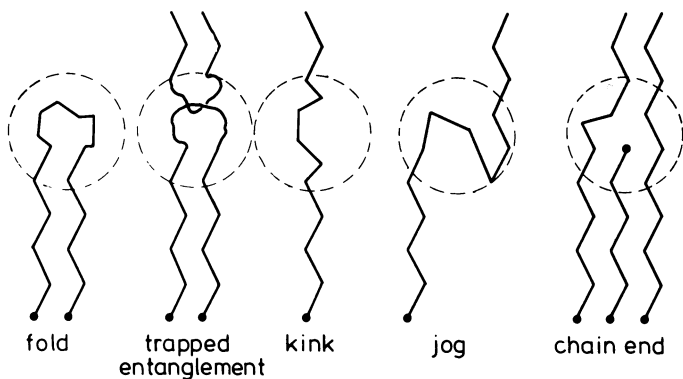
Dislocations in polymers
