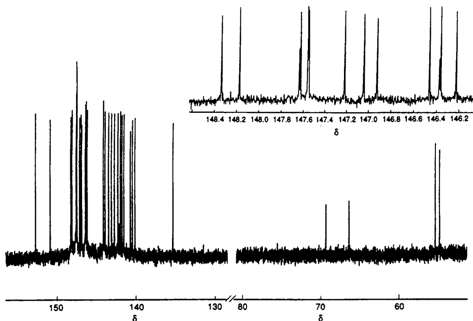
Fig. 4 The ^{13}C NMR spectrum of C_{60}Cl_6 .
