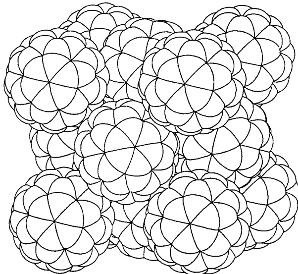
Fig. 2 Space filling representation of the face-centred cubic packing of pure C_{60} .
