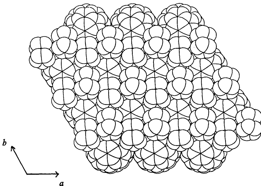
Fig. 6 Space-filling representation of the structure of C_{60}.2(Cp_2Fe) ; view perpendicular to the ab plane showing how the Cp_2Fe molecules are arranged on the close-packed layer of C_{60} molecules.
