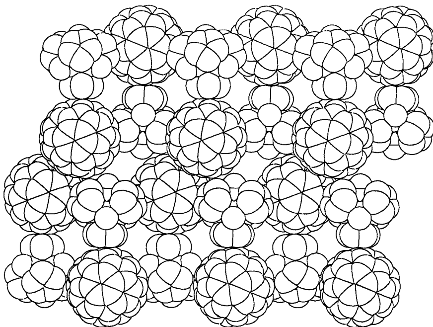
Fig.7 Space-filling representations of the C_{60}.Cp_4Fe_4(CO)_4 host lattice structure; view perpendicular to bc plane ( C_6H_6 molecules omitted for clarity). The double-columnar stacks of C_{60} molecules are perpendicular to the plane of the paper (along a axis).
