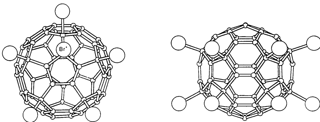
Fig. 3 The molecular structures of C_{60}Br_6 and C_{60}Br_8 .
