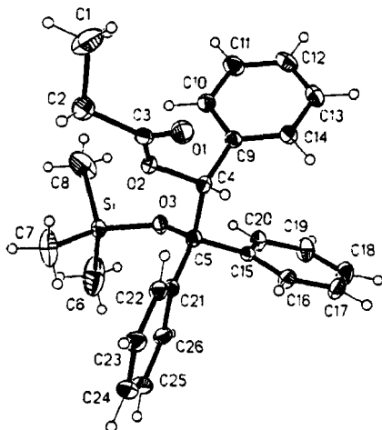
Fig. 1: X-Ray Structure of 8a
