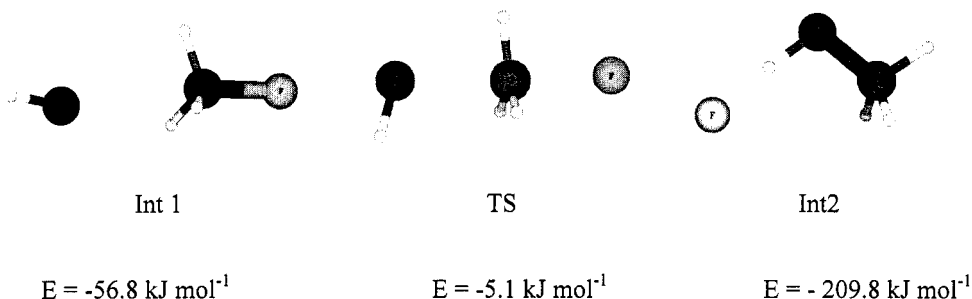
Figure 4: Optimized structures and relative energies (assuming the reagents as E = 0 ) for the intermediates and transition state of reaction (6) calculated at the MP2/6-311++G(3dp,3df)//MP2/6-311++G(3dp,3df) level with ZPE corrections.
