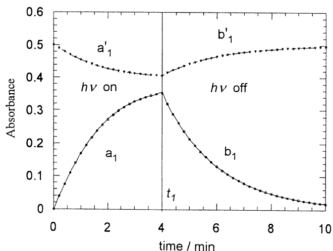
Fig. 1 Evolution of the absorbance at two wavelengths of a unimolecular photochromic system under continuous irradiation. Curves a_1 and b_1 are monitored at the \lambda_{\max} of the open form, while a'_1 and b'_1 are at the irradiation wavelength ( \lambda_{\text{irr}} ). UV irradiation has been stopped at time t_1 . The thermal rate constant k_{\text{BA}} is extracted from the relaxation processes ( b_1 and b'_1 from t_1 \rightarrow \infty ) in the dark, while \Phi_{\text{AB}} and \varepsilon_{\text{B}} are extracted from the kinetic curves under irradiation ( a_1 and a'_1 corresponding to the irradiation periods 0-t_1 ). Knowledge of the evolution of the absorbance at the irradiation wavelength ( \lambda_{\text{irr}} ) allows the fraction of incident photon flux that is really absorbed by the photochromic starting compound A to be calculated.
