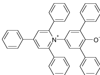
2,6-diphenyl-4-(2,4,6-triphenyl-1-pyridinio)phenoxide
