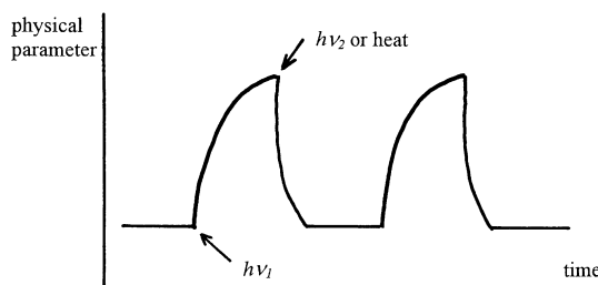
Fig. 2 Photoinduced cyclic variation of a physical property in a photoresponsive system.
