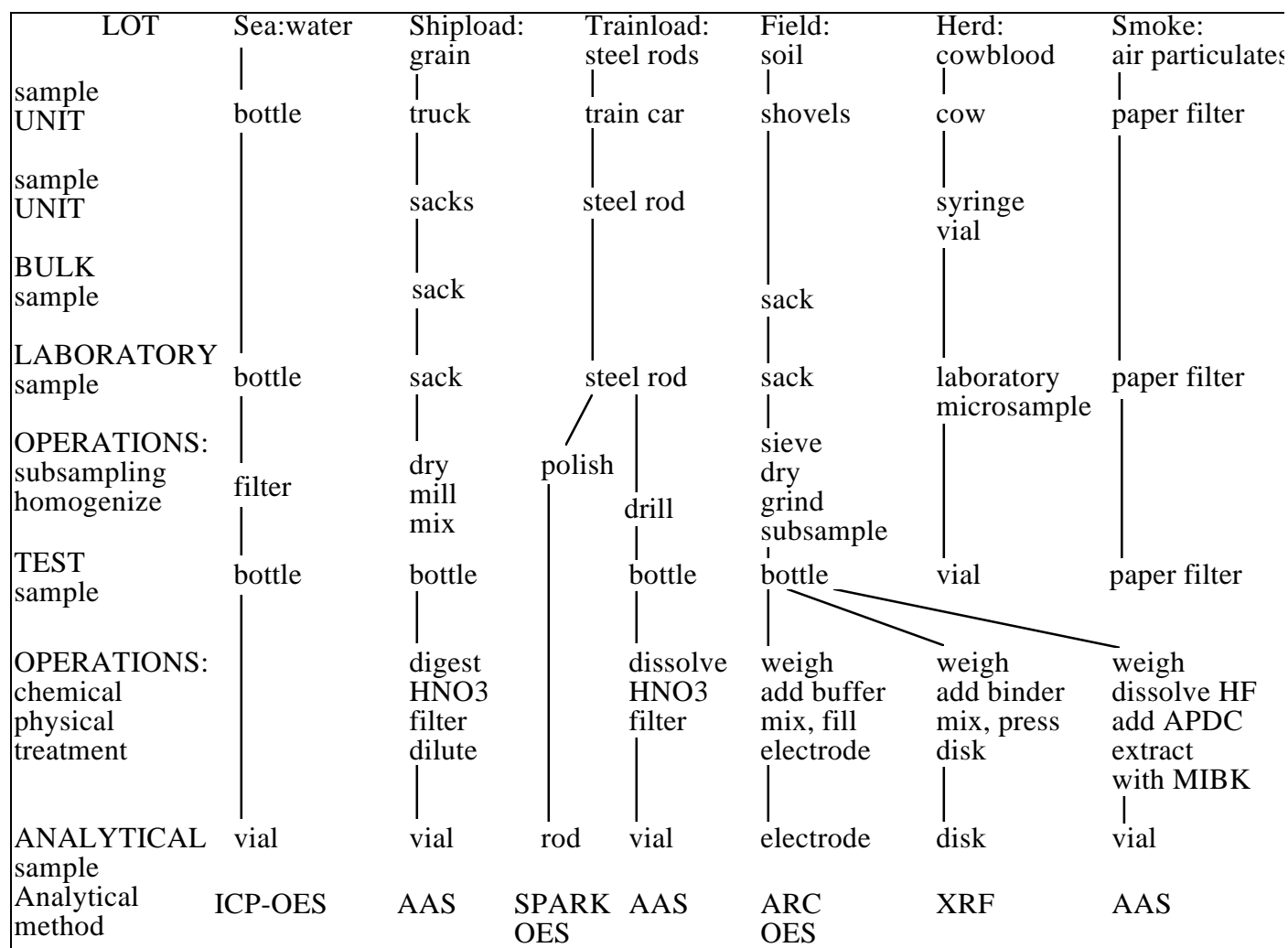
Fig. X.2 Examples of routes from sample to analysis illustrating sampling terminology. ICP: Inductively Coupled Plasma; XRF: X-ray Fluorescence; ADPC: Ammonium Pyrrolidine Dithiocarbamate; MIBK: Methyl Isobutyl Ketone; AAS: Atomic Absorption Spectrometry; OES: Optical Emission Spectrometry
