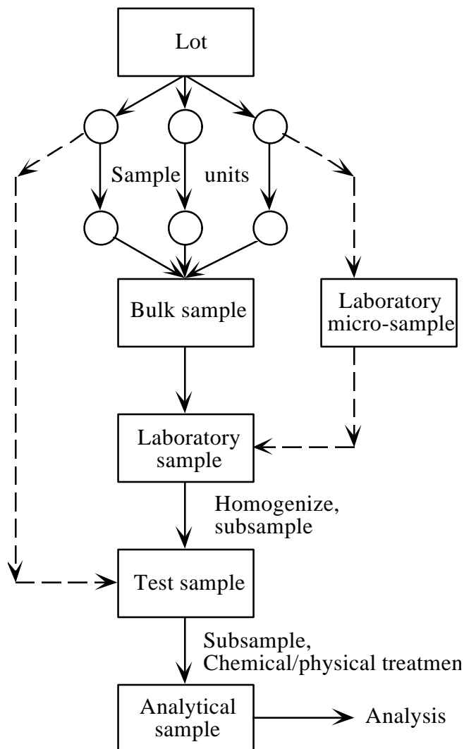
Fig. X.1 Schematic diagram of sampling stages and terminology
