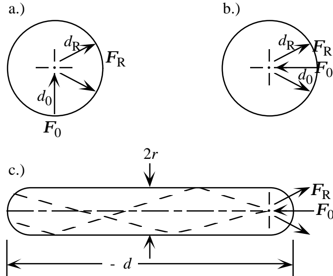
Fig. 6. Liquid sample arrangements: a.) perpendicular-scattering (90°) arrangement in a spherical cell, b.) back-scattering (180°) arrangement in a spherical cell, and c.) back-scattering arrangement through the spherical bottom of a capillary cell (see ref. 1).
