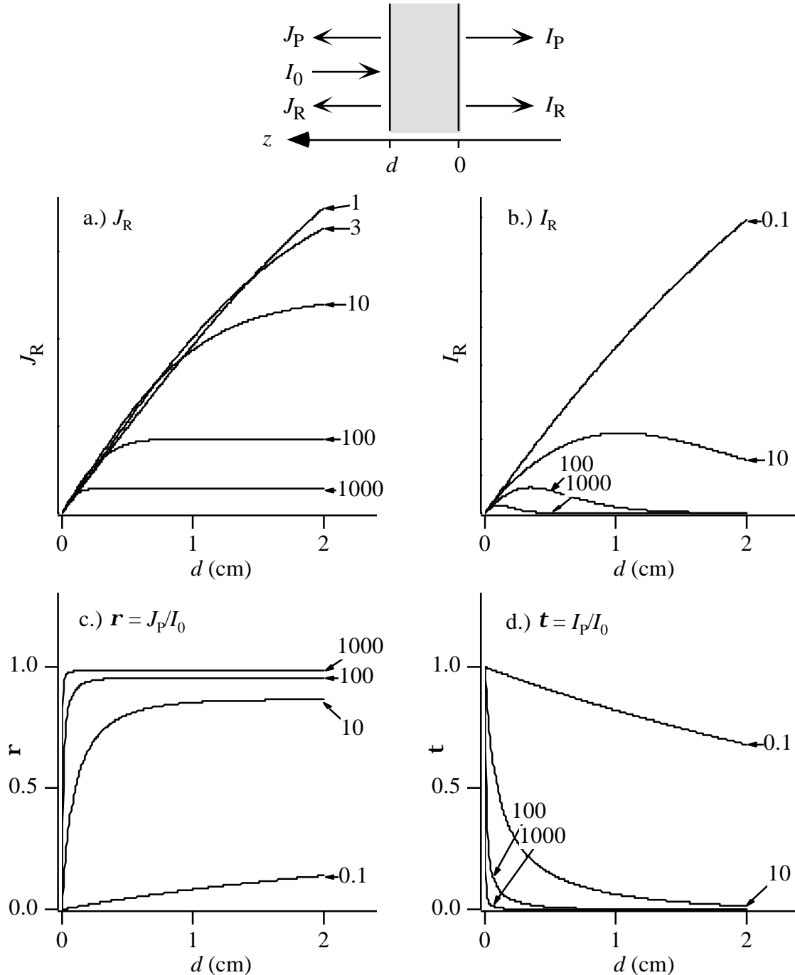
Fig. 5. Plots of the forward ( I ) and backscattered ( J ), unshifted (P) and Raman (R) intensities versus sample thickness d and at several values of r , for a = 0.1 \text{ cm}^{-1} . The incident intensity is I_0 . Plot a.) is of J_R the back-scattered Raman intensity; b.) is of I_R , the forward-scattered Raman intensity; c.) is of r , the reflectance of the Rayleigh radiation; and d.) is of t , the transmittance of the Rayleigh radiation.
